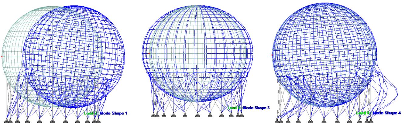
Fig.(2): Mode Shapes of LPG spherical Tank for First Four Modes
