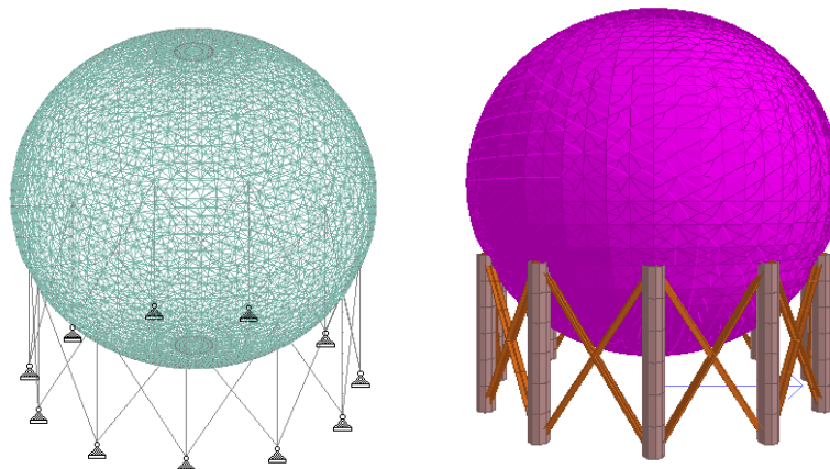
Fig.(6): Finite Element 3D Model Of LPG Spherical Tank
