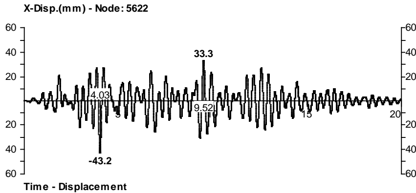
Fig.(7): Maximum Lateral Displacement Response versus Time
