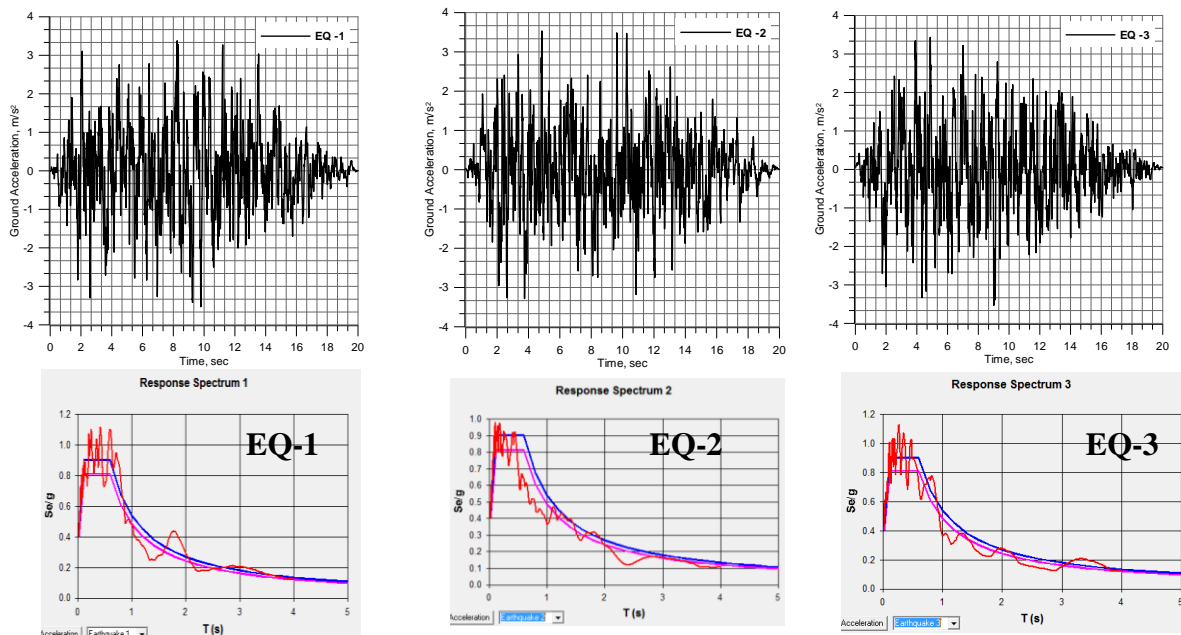
Fig.(5): Acceleration-Time Histories of Artificial Earthquakes and Its Spectra
