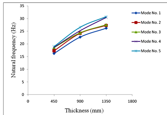
Fig. (10): Effect of thickness variation on natural frequencies of empty buried tank
