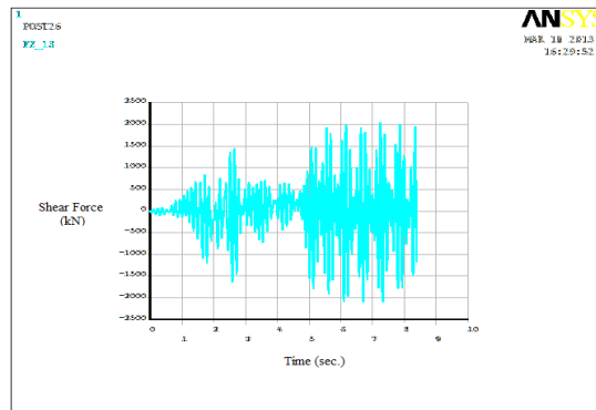
Fig.(15): Shear force for empty tank under ground
